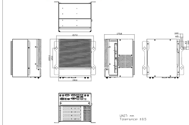
TB-5745-MVS X4 Expansion with Wall Mount (standard)
