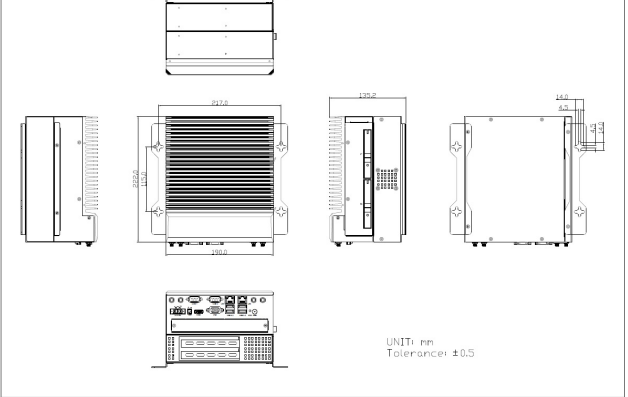
TB-5745-MVS X2 Expansion with Wall Mount (standard)
