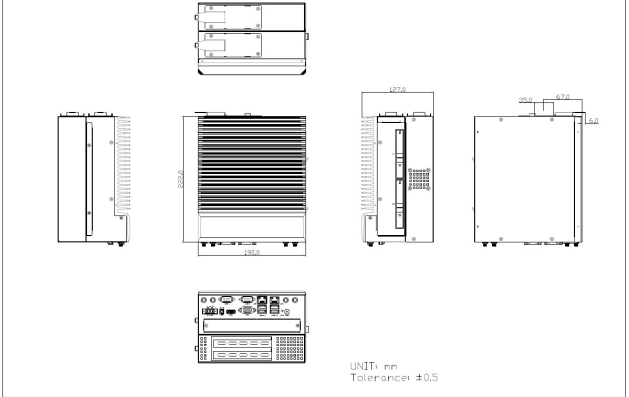
TB-5745-MVS X2 Expansion with DIN Mount (option)
