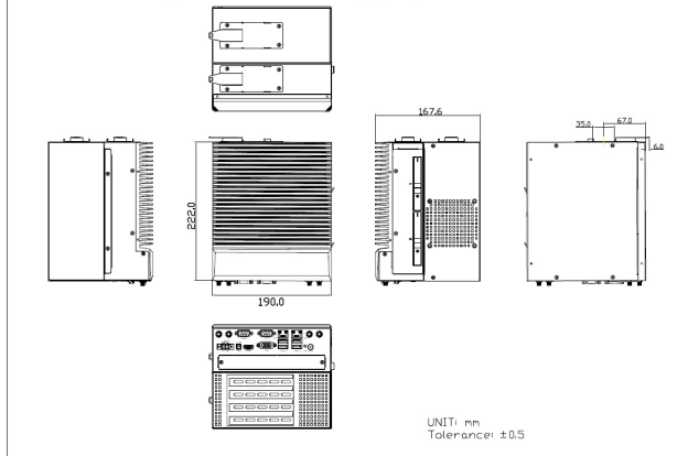
TB-5745-MVS X4 Expansion with DIN Mount (option)
