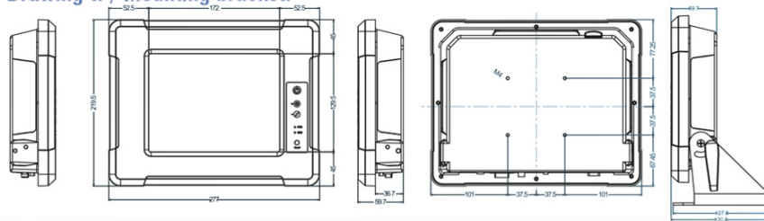
Drawing w / Mounting bracket:
