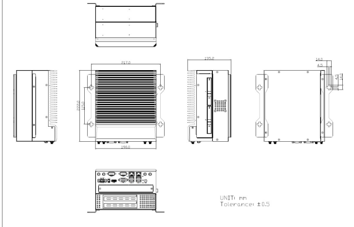
TB-5745-MVS X2 Expansion with Wall Mount (standard)
