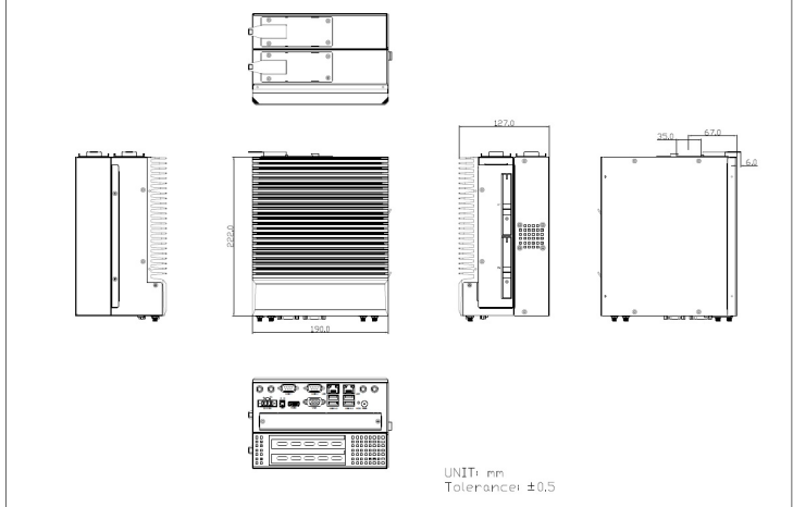
TB-5745-MVS X2 Expansion with DIN Mount (option)
