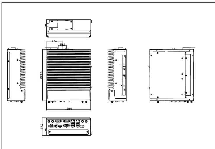
TB-5745-MVS (no expansion) with DIN Mount (option)
