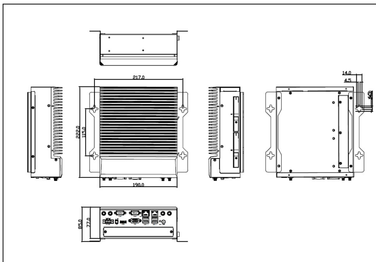
TB-5745-MVS (no expansion) with Wall Mount (standard)
