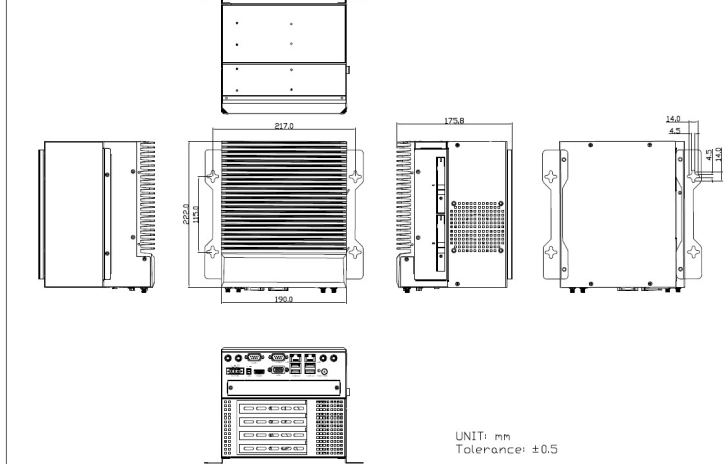
TB-5745-MVS X4 Expansion with Wall Mount (standard)
