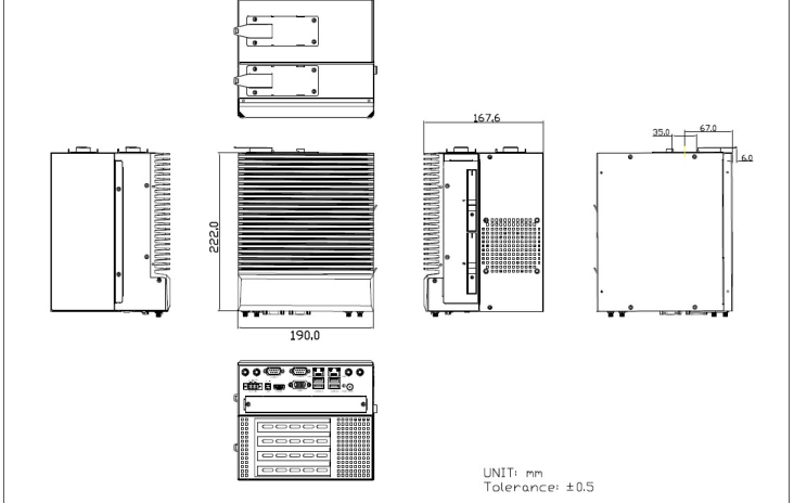
TB-5745-MVS X4 Expansion with DIN Mount (option)
